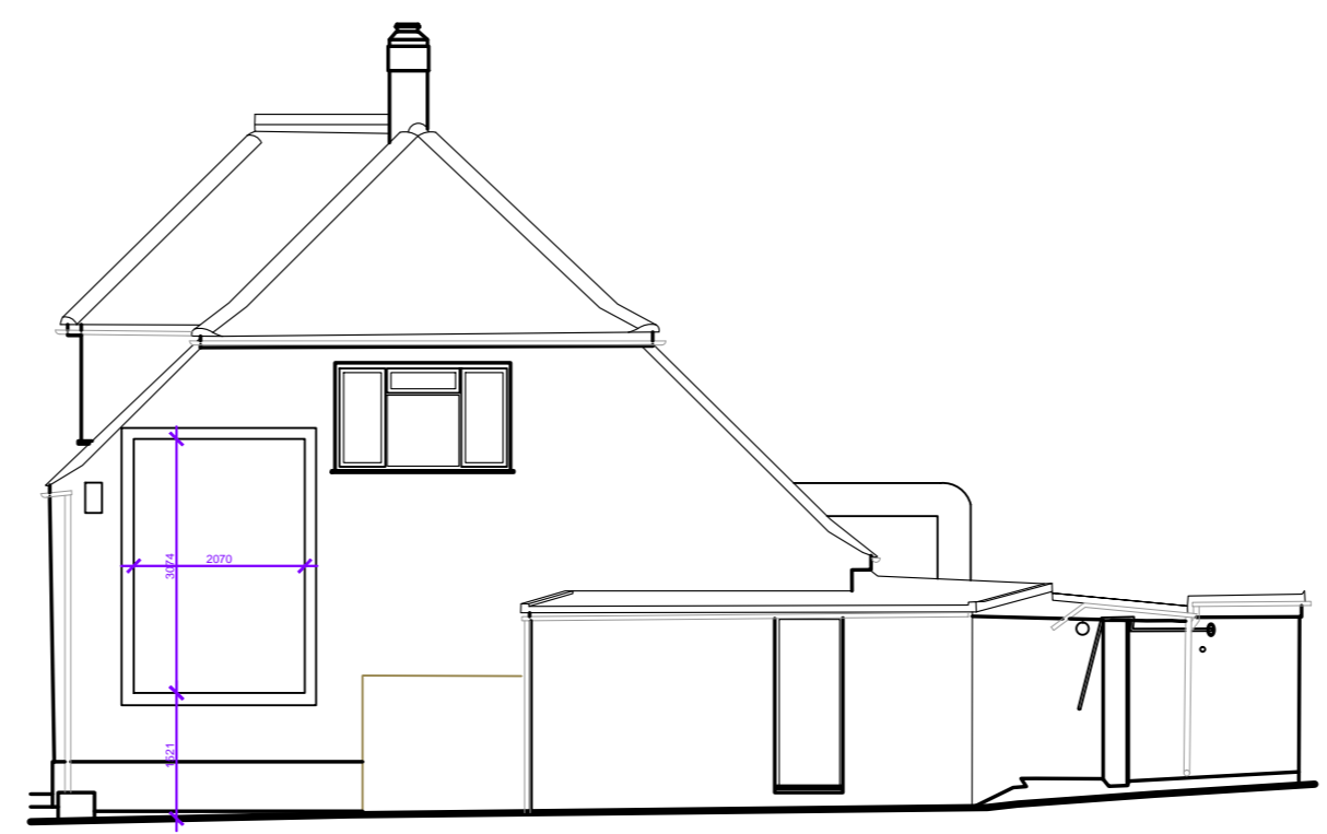
Side Elevation Datum 49.00m
