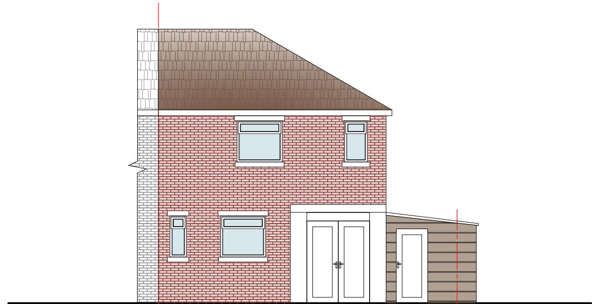
REAR ELEVATION Sc.1:100
