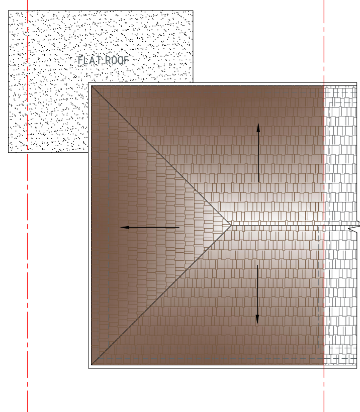
ROOF PLAN Sc.1:100
