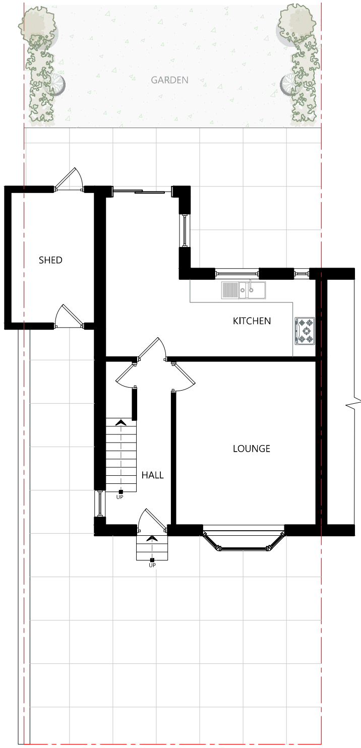
GROUND FLOOR PLAN Sc.1:100
