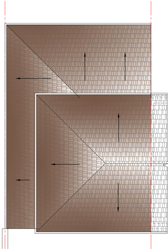
ROOF PLAN Sc.1:100
