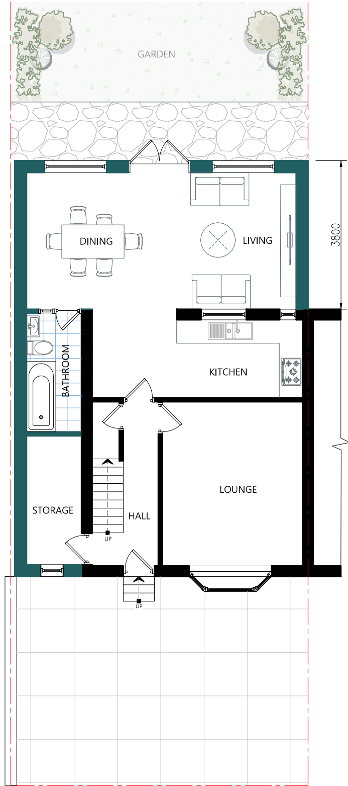
GROUND FLOOR PLAN Sc.1:100
