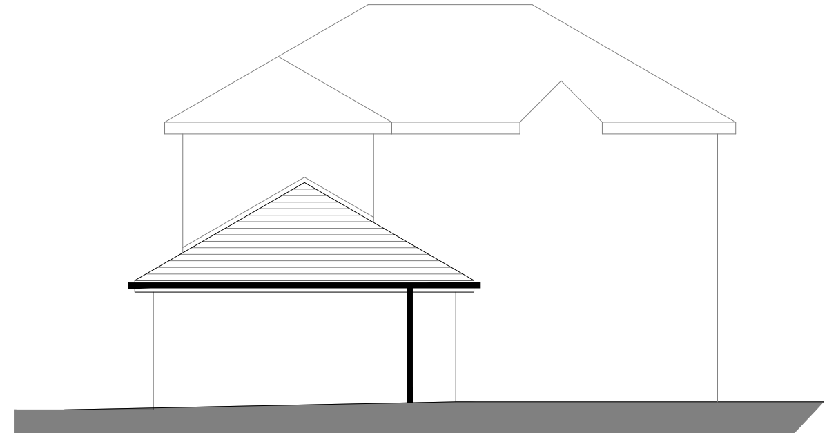
Existing side elevation facing south west 1:100
