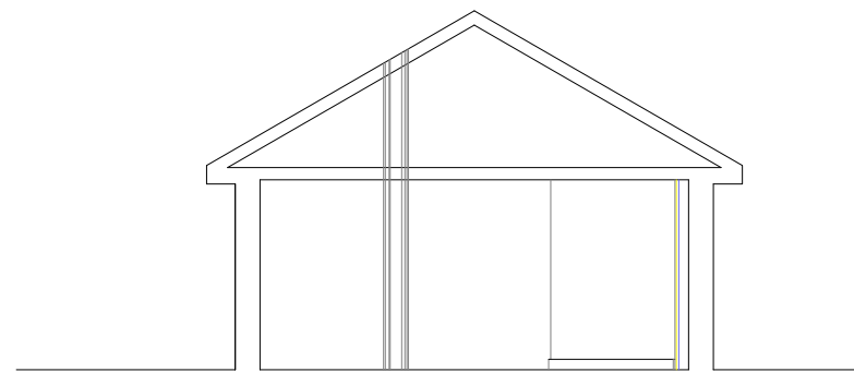
Proposed section 1 : 1 0 0
