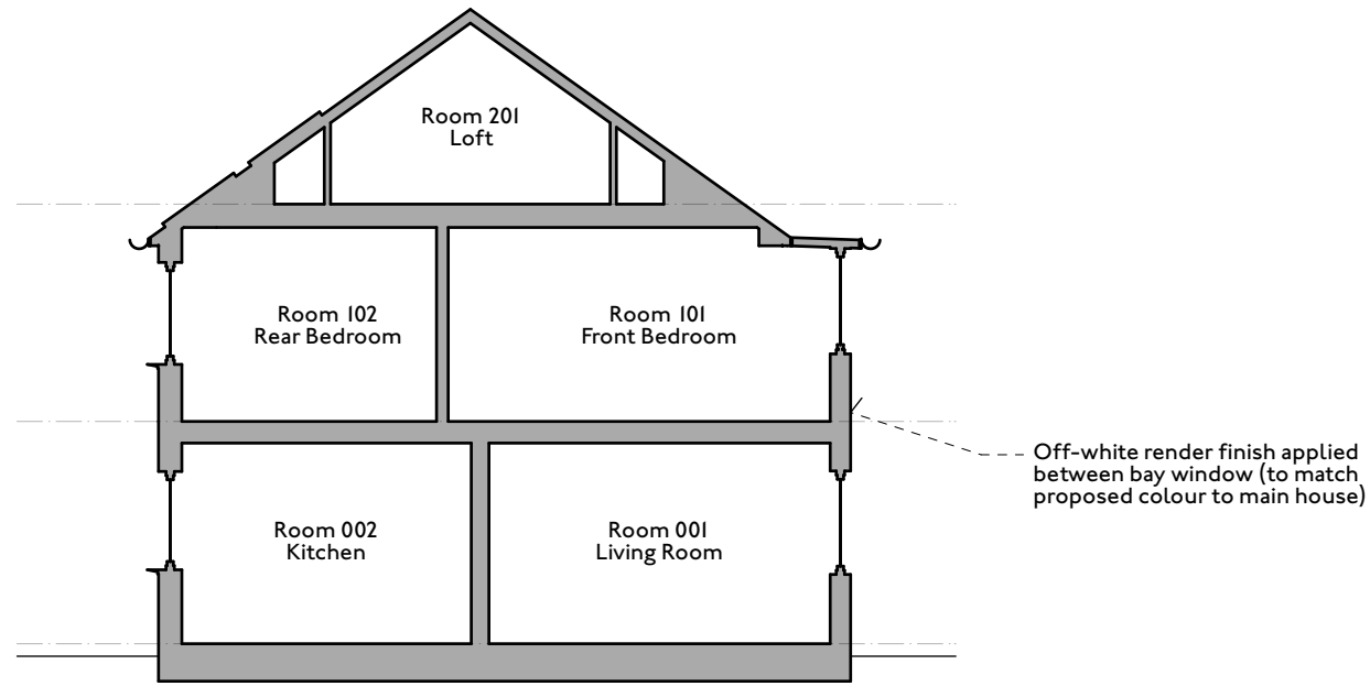
1 | 1:100 Section AA
