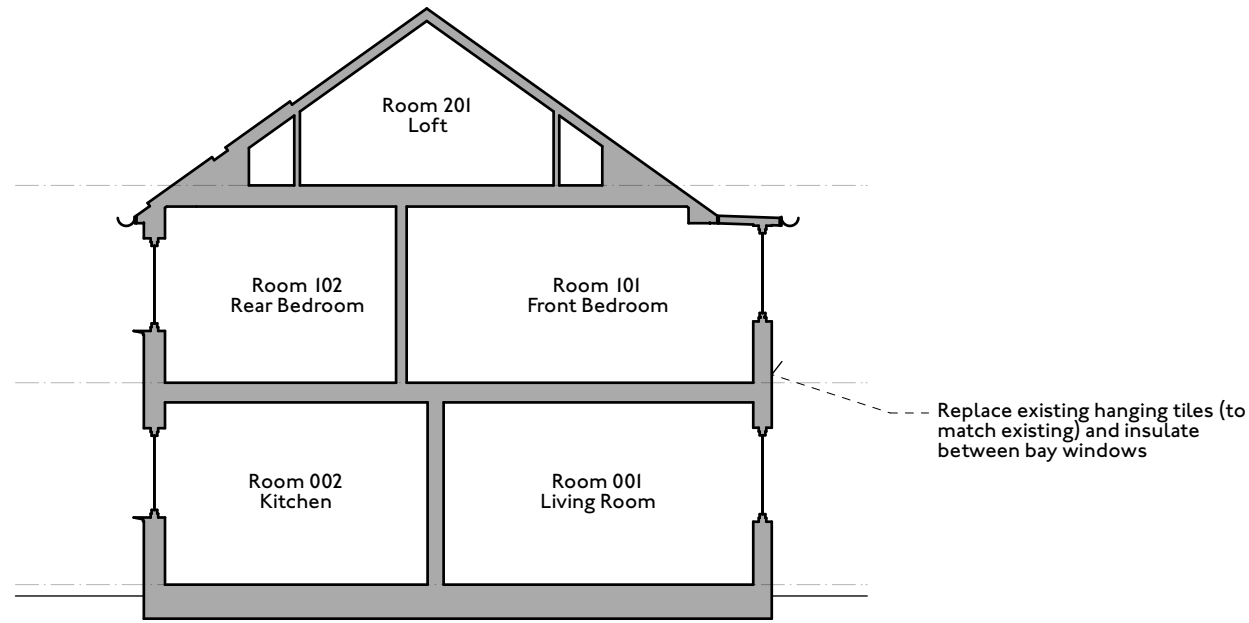
1 | 1:100 Section AA
