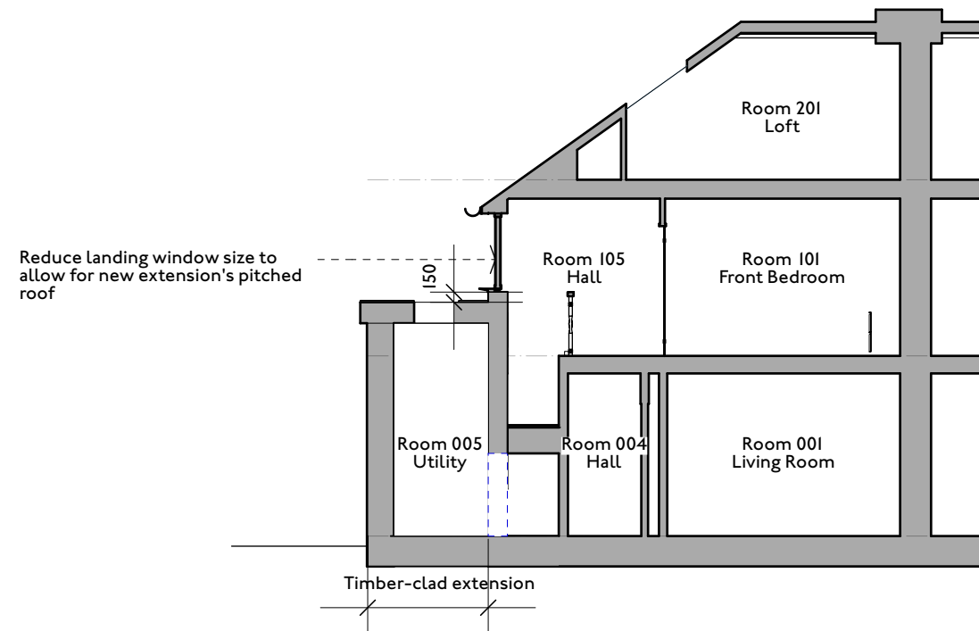
2 | 1:100 Section BB
