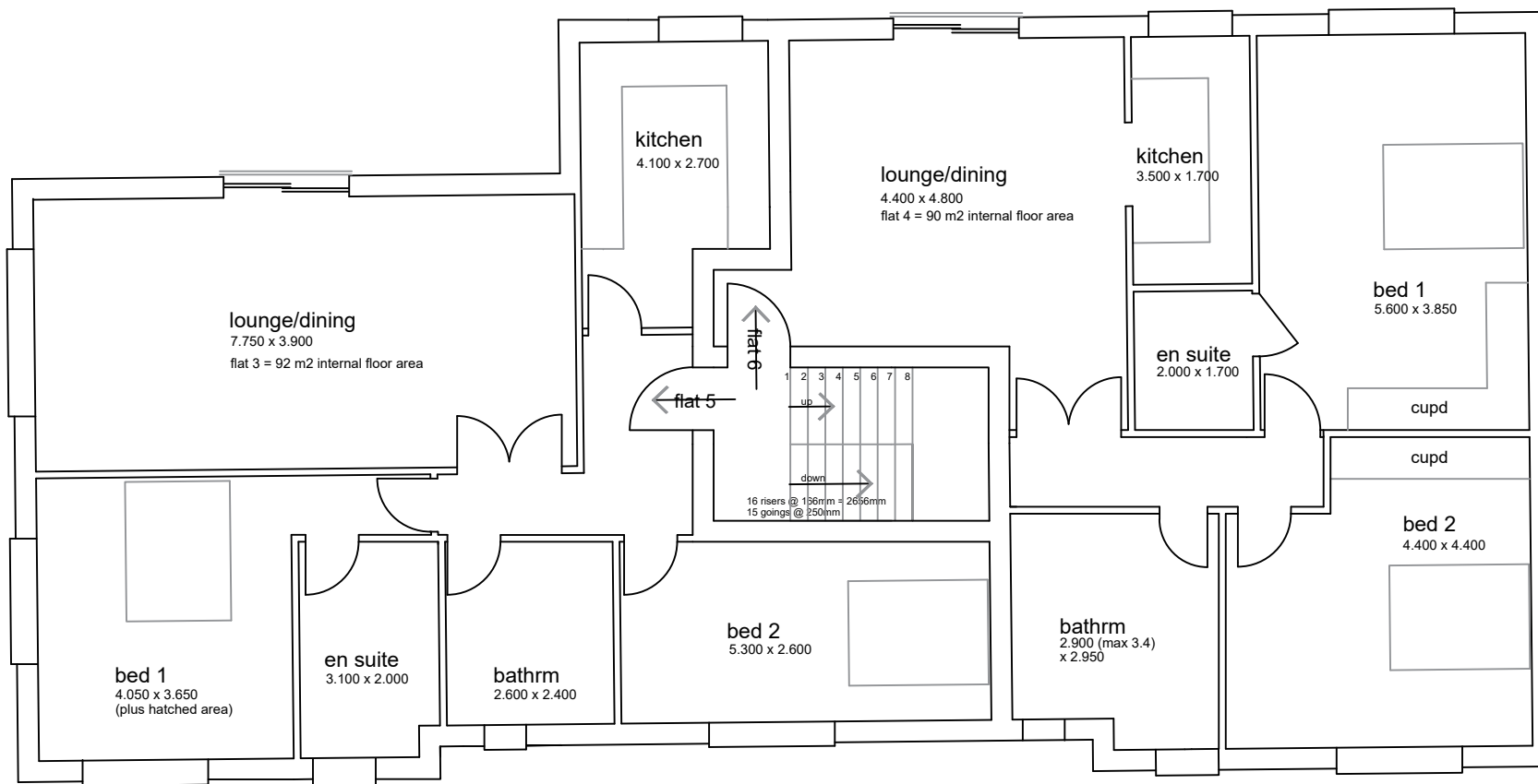
second floor plan - scale 1:100
