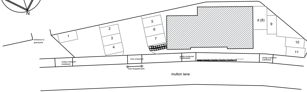
proposed site layout - 114 mutton lane, potters bar - scale 1:500 1 2 3 4 5 6 7 8 9 10 metre scale bar
