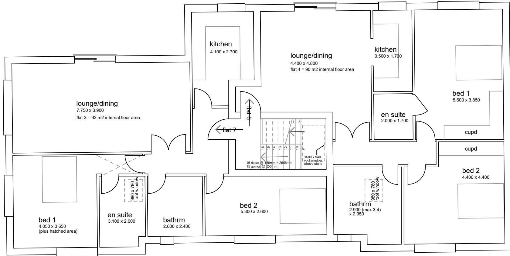
third floor plan - scale 1:100
