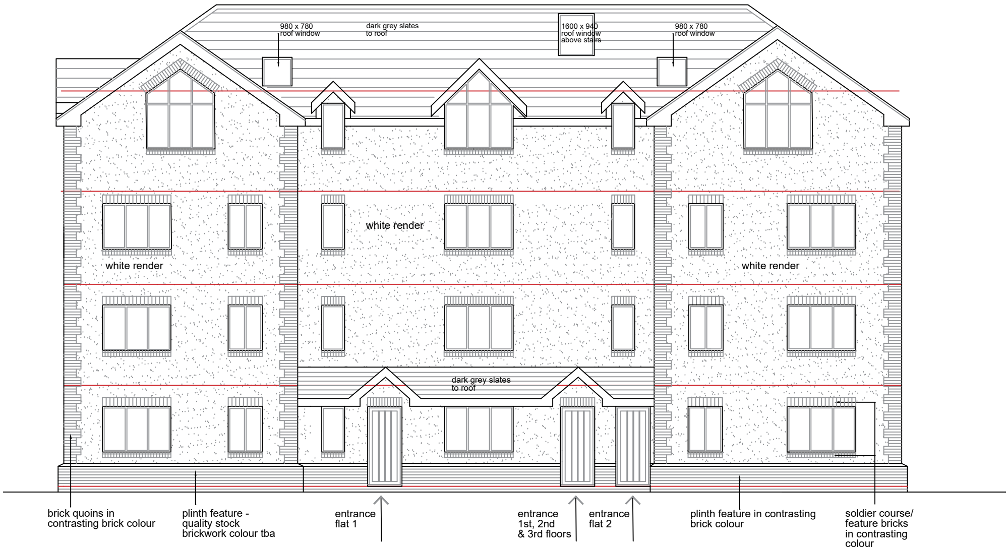
proposed front elevation - scale 1:100 114 mutton lane, potters bar
