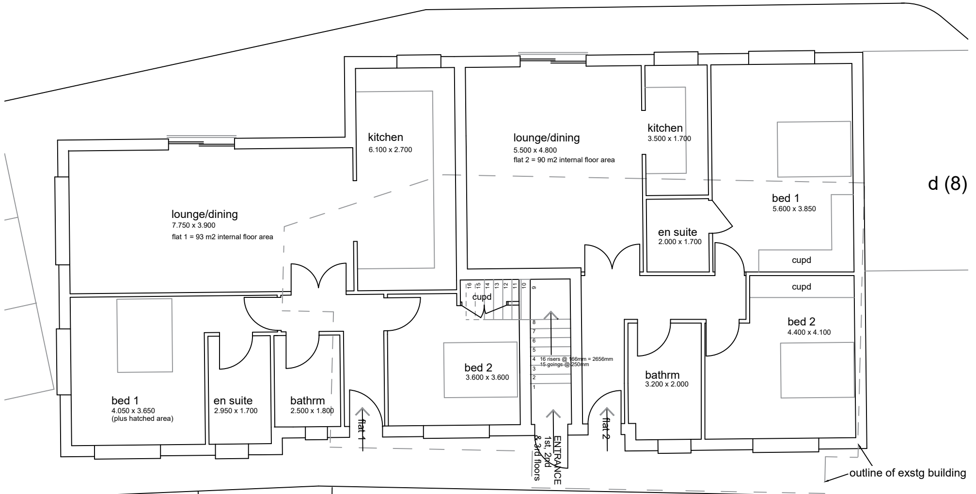
proposed ground floor plan - 114 mutton lane, potters bar - scale 1:100
