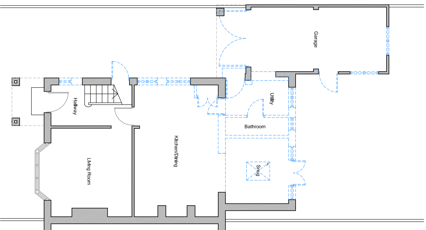
02. Demolition Ground Floor Plan
