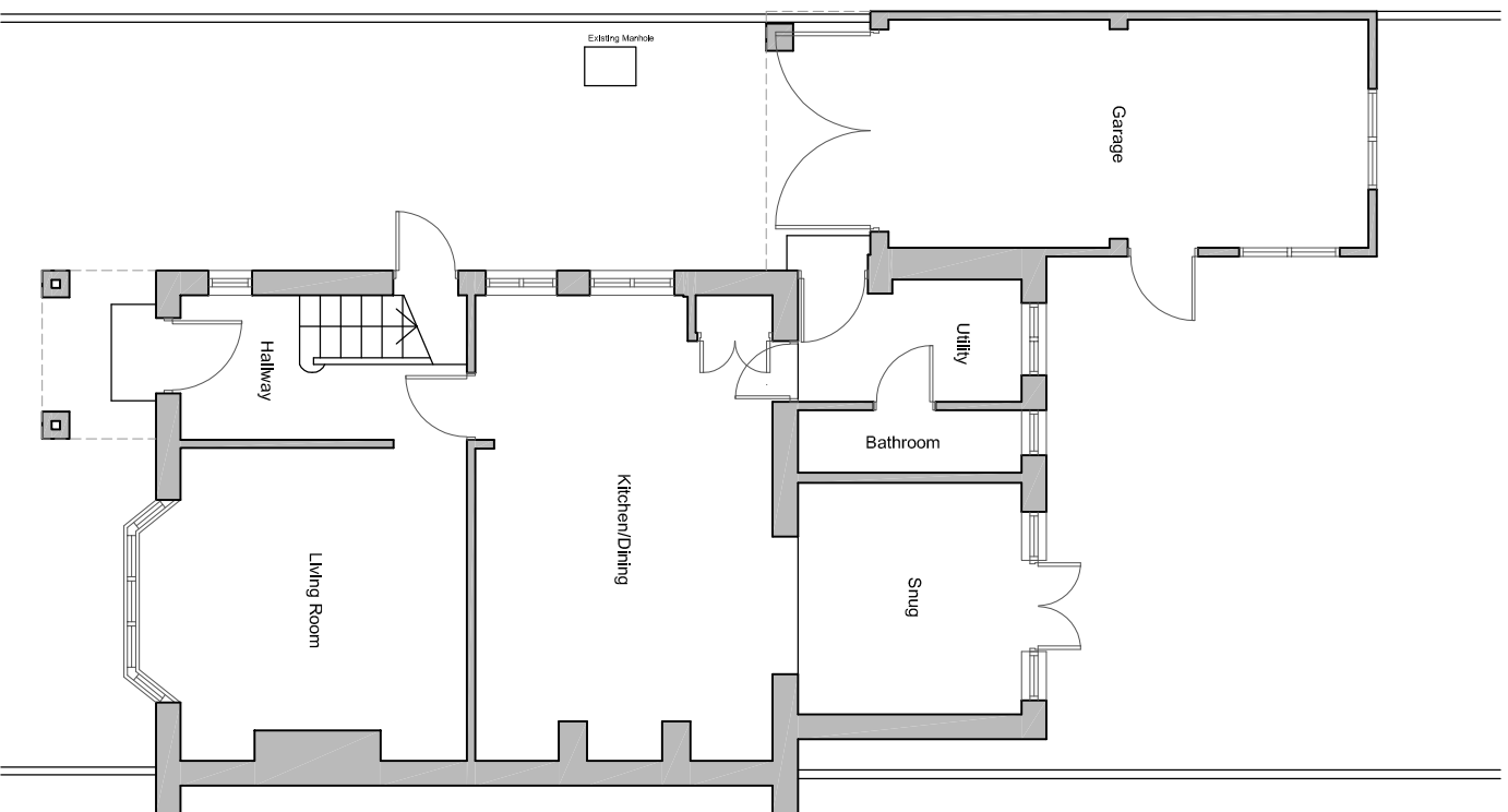
01. Existing Ground Floor Plan
