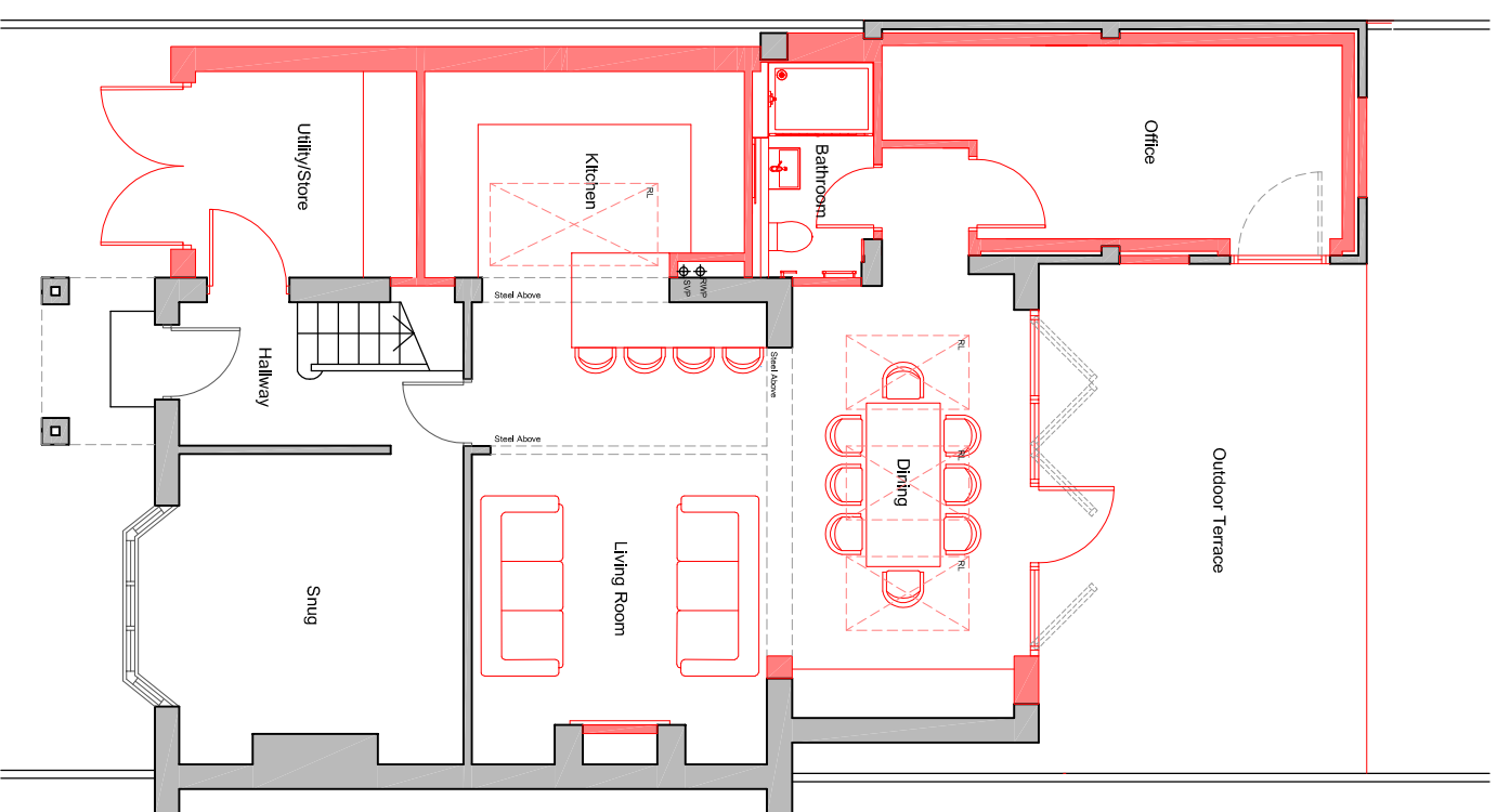
03. Proposed Ground Floor Plan
