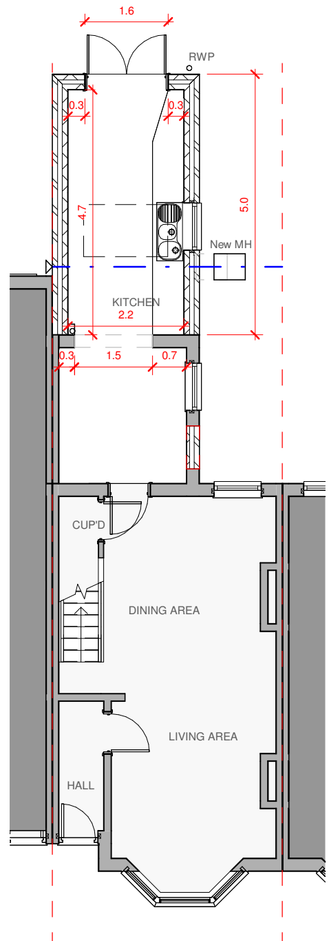
01 Proposed Ground Floor. 1 : 100
