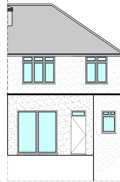
REAR ELEVATION, EXISTING PLAN, SCALE 1:100
