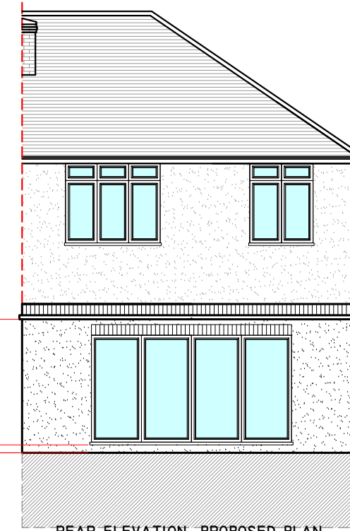
REAR ELEVATION, PROPOSED PLAN, SCALE 1:100
