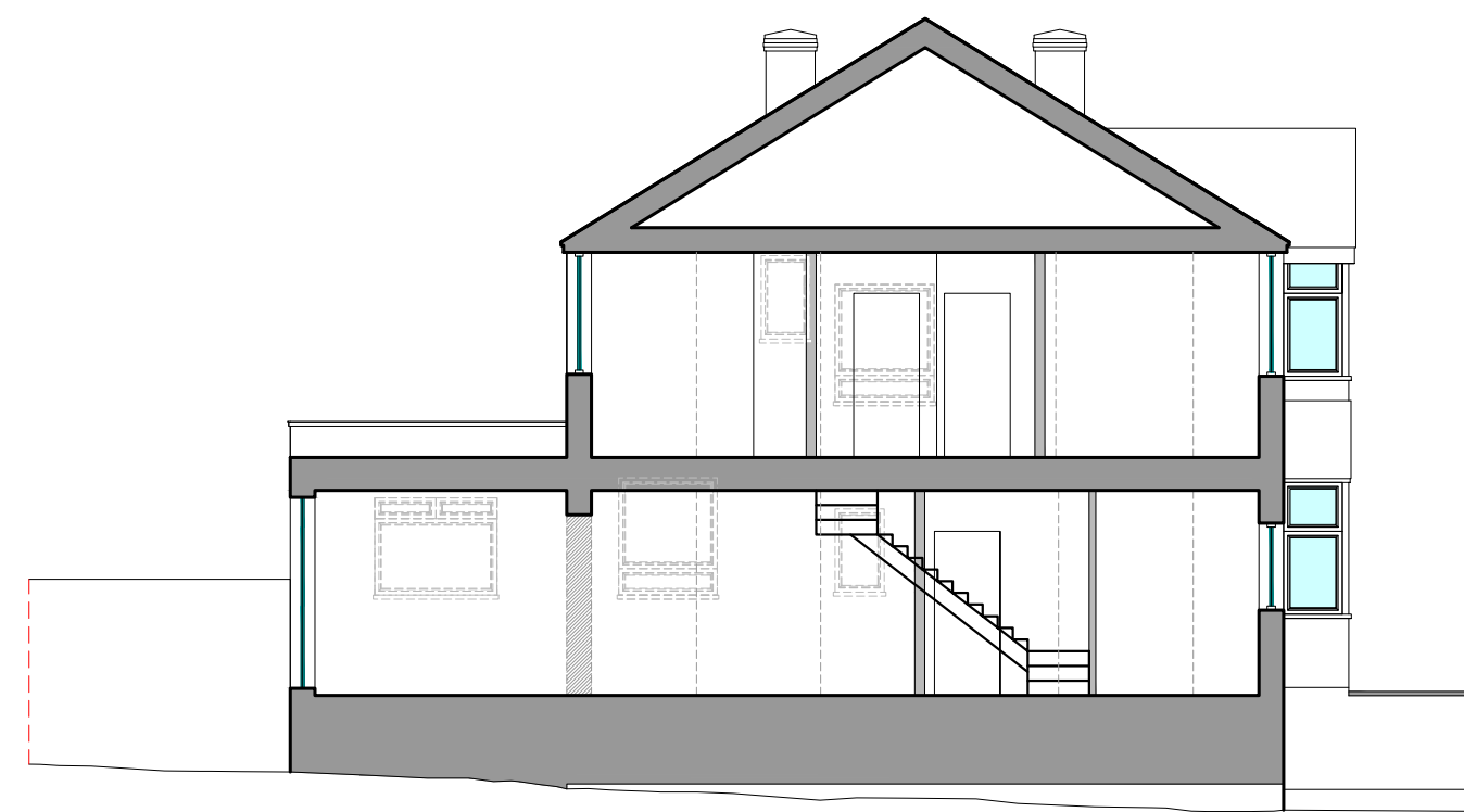
SIDE ELEVATION, EXISTING SECTION, SCALE 1:100
