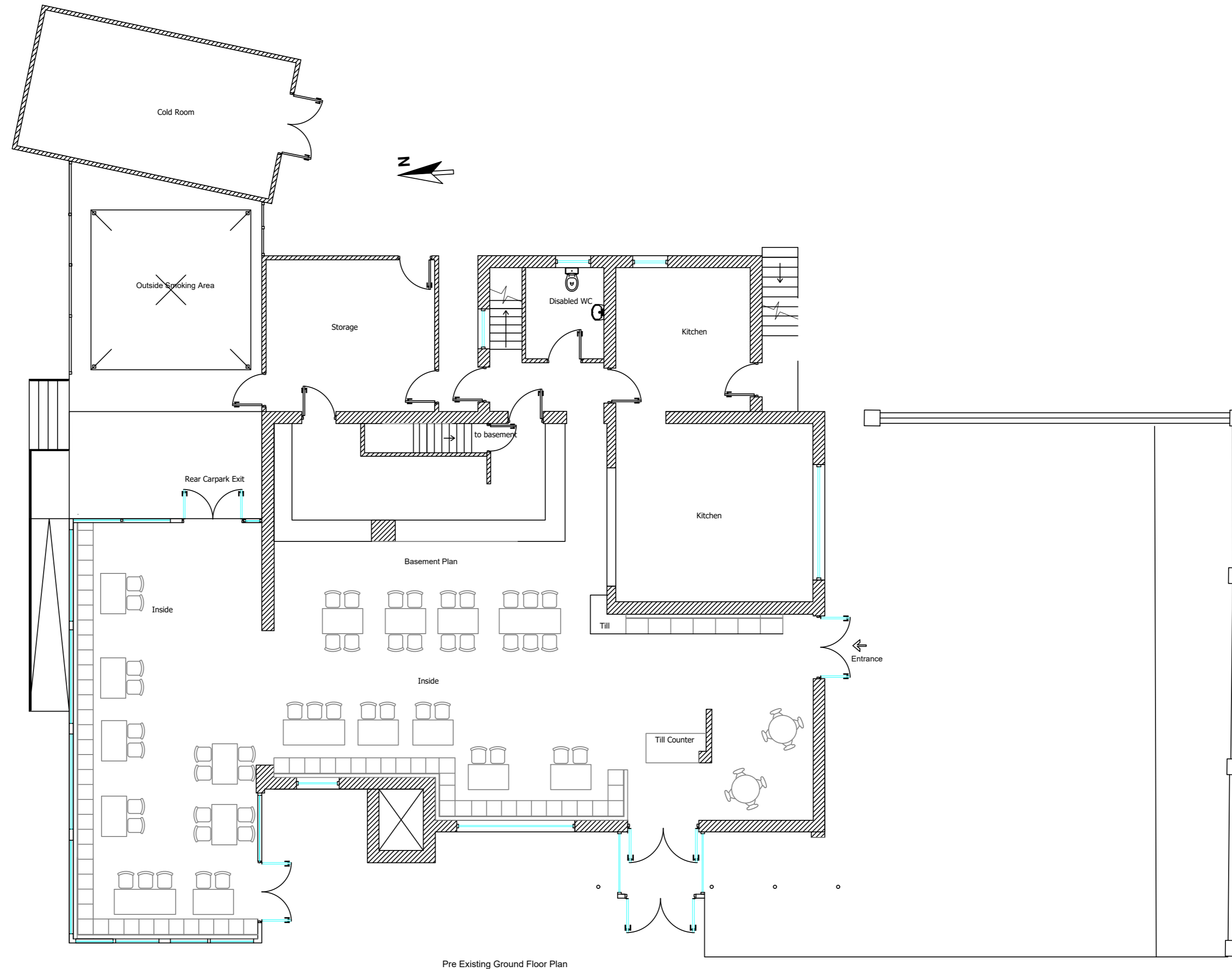
Pre Existing Ground Floor Plan
