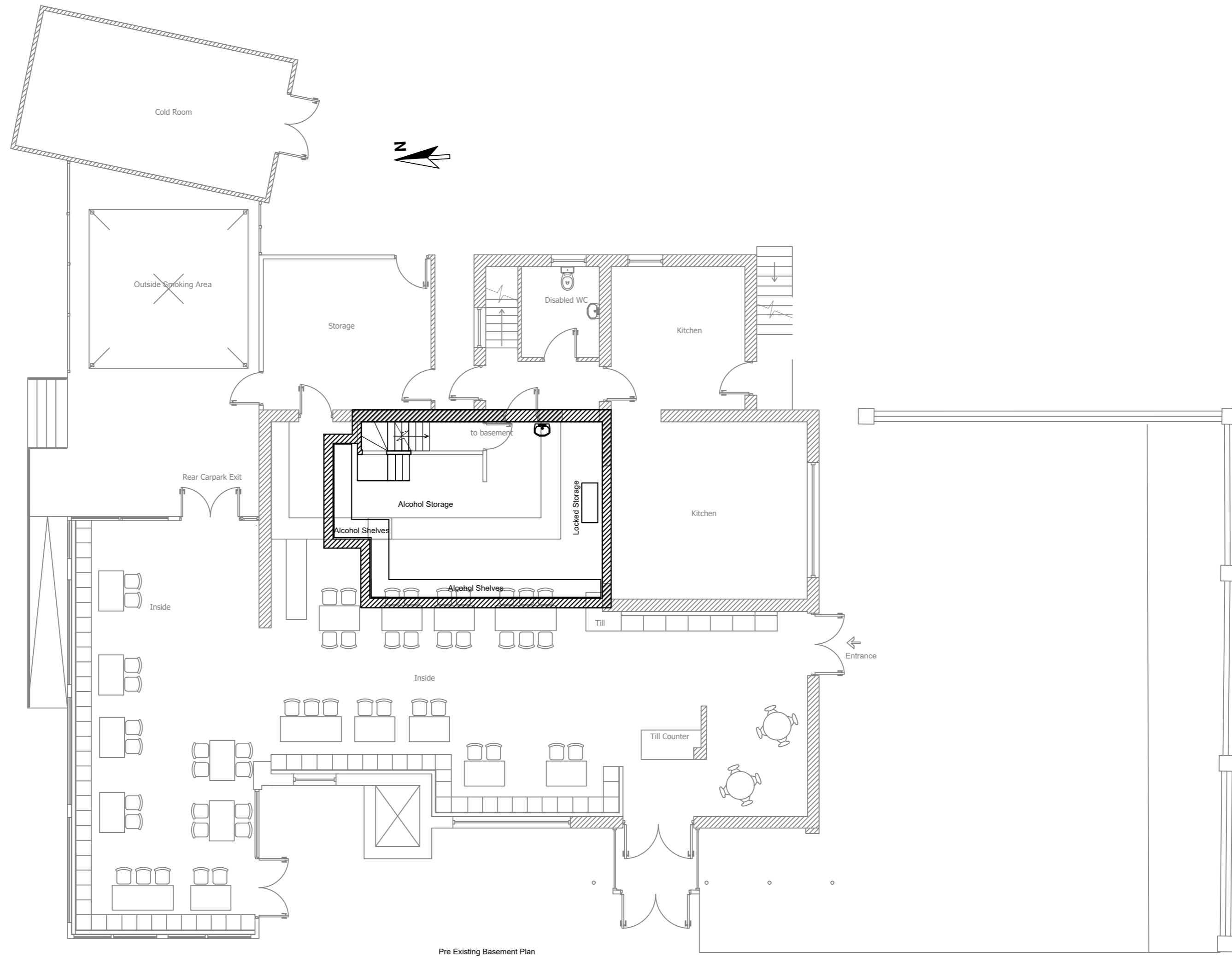
Pre Existing Basement Plan
