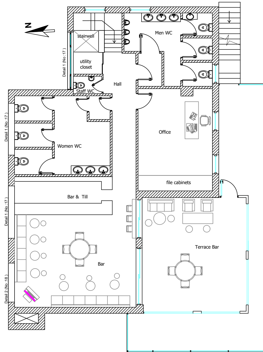
Pre Existing First Floor Plan
