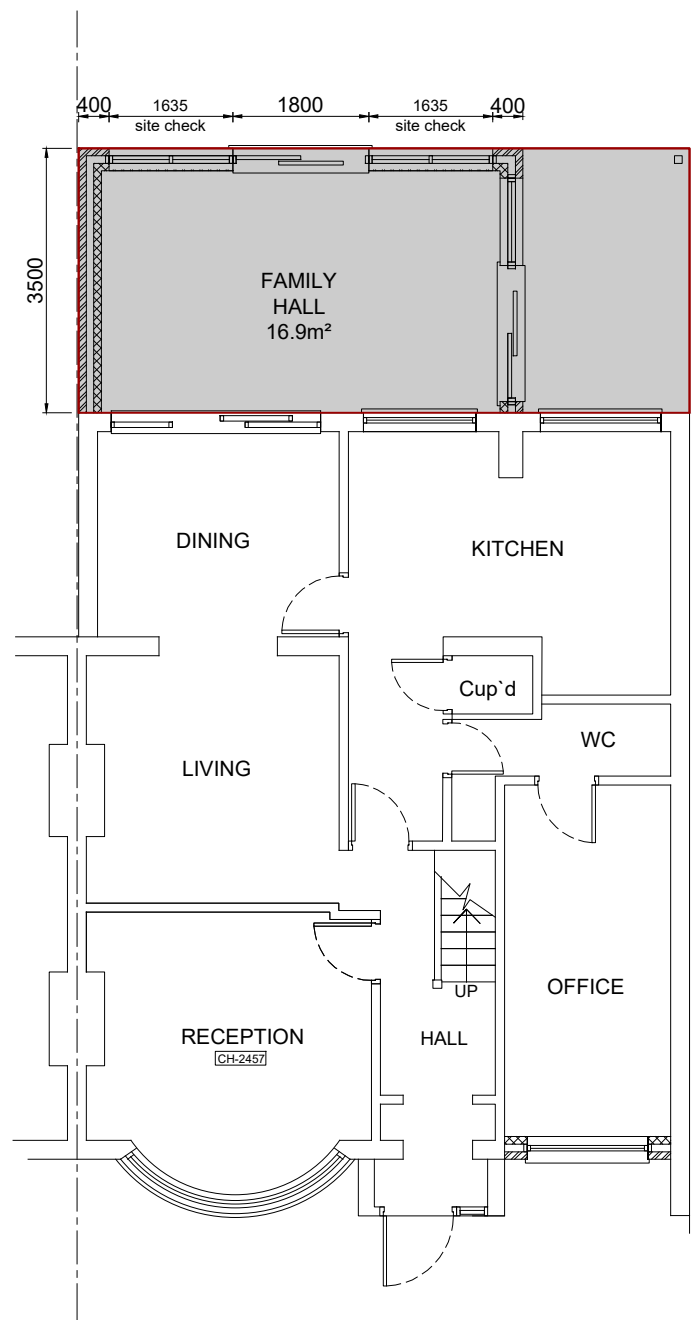
GROUND FLOOR PLAN 1:100 Previously APPROVED Planning Ref: 22/02706/FUL
