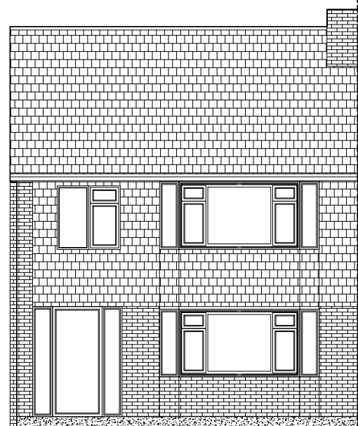
FRONT ELEVATION
