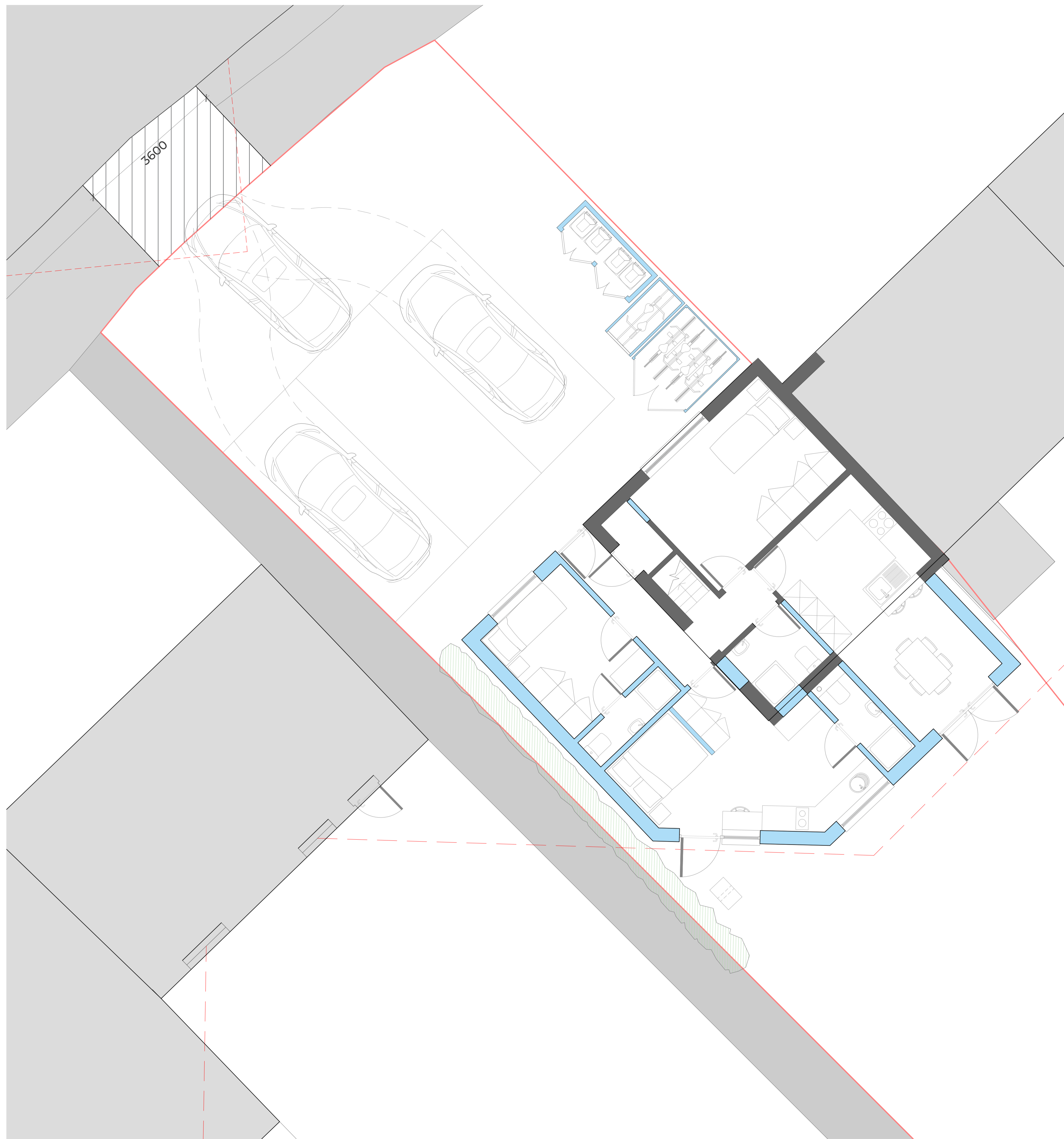
Proposed Site Plan 1:50
