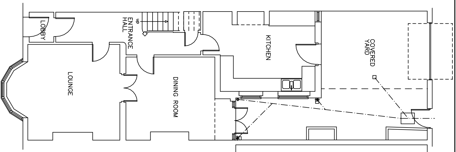
GROUND FLOOR
