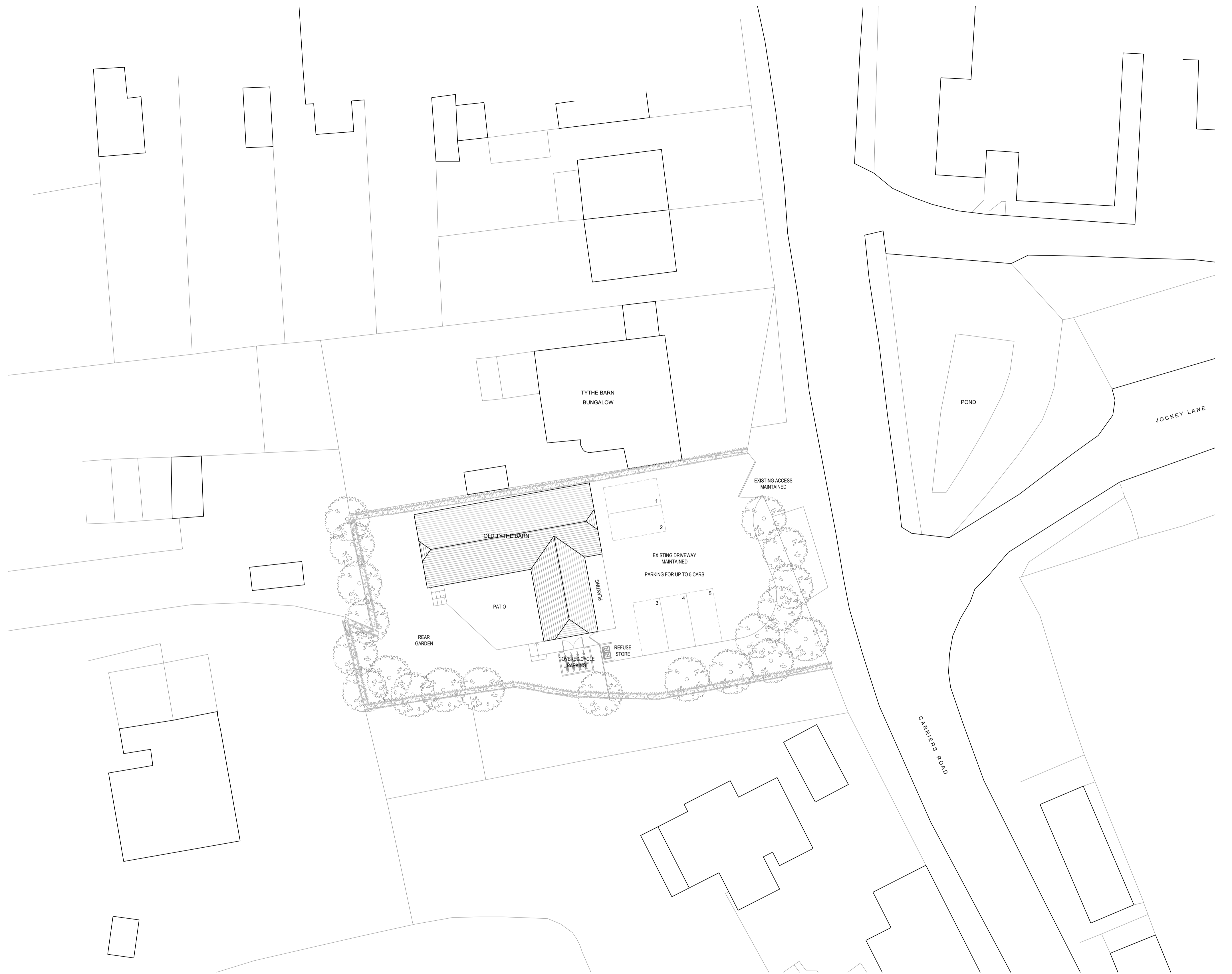
PROPOSED BLOCK PLAN SCALE 1:200
