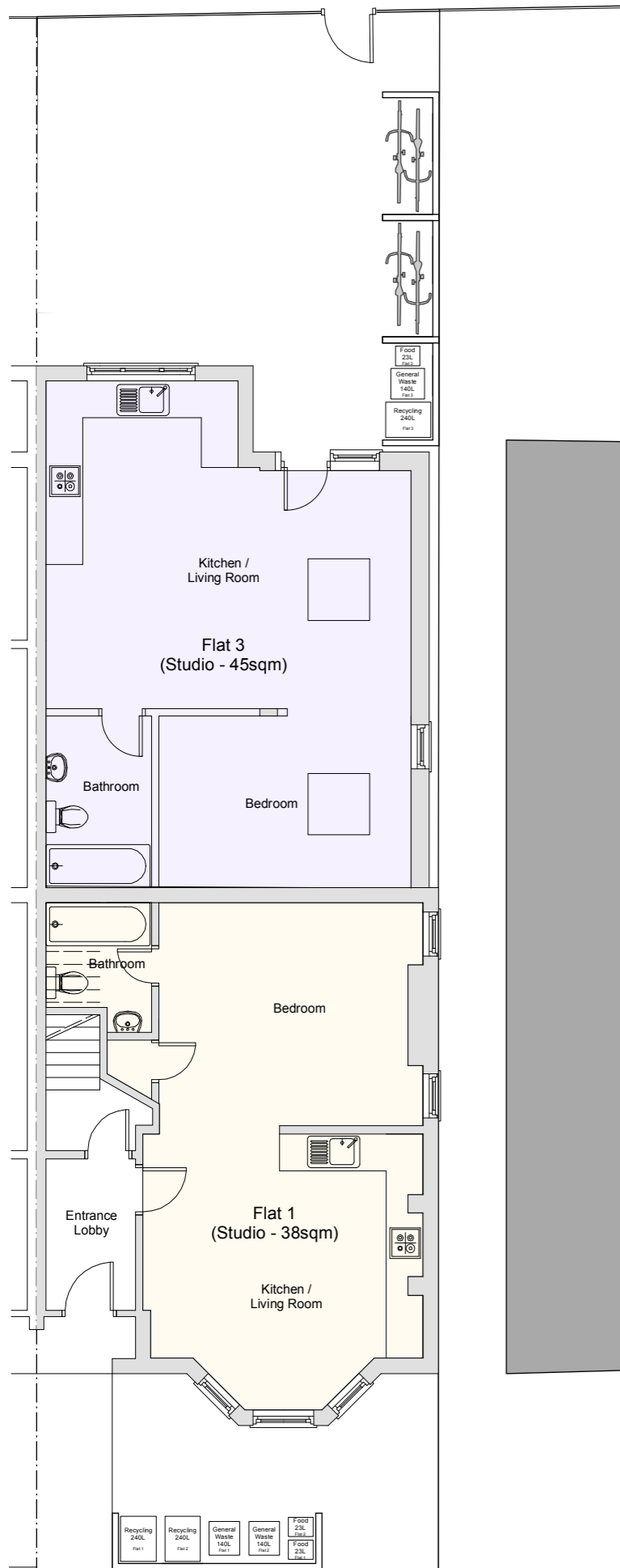
Proposed Ground Floor Plan (Flat 1 & 3)
