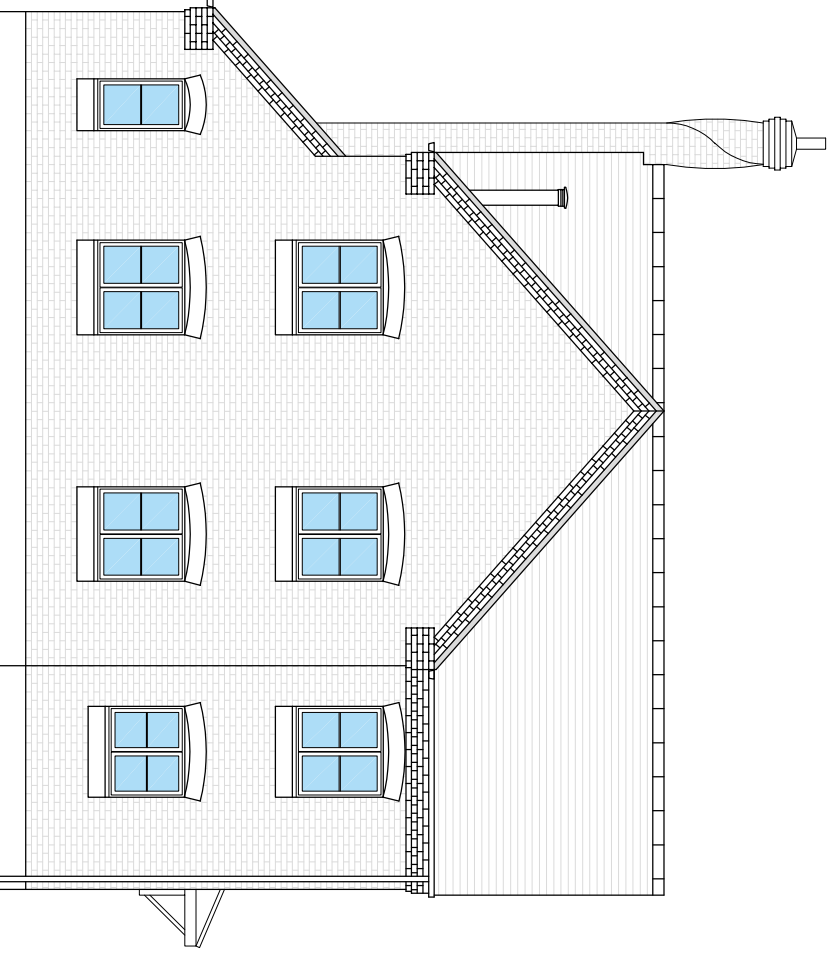
Rear Elevation
