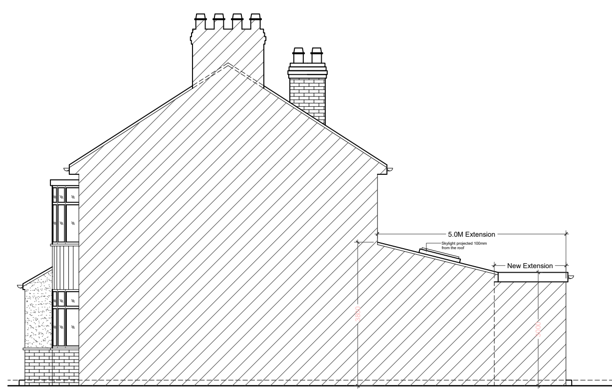
04 - SIDE ELEVATION
