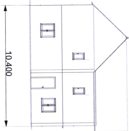
South elevation
