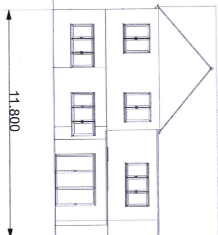
East elevation
