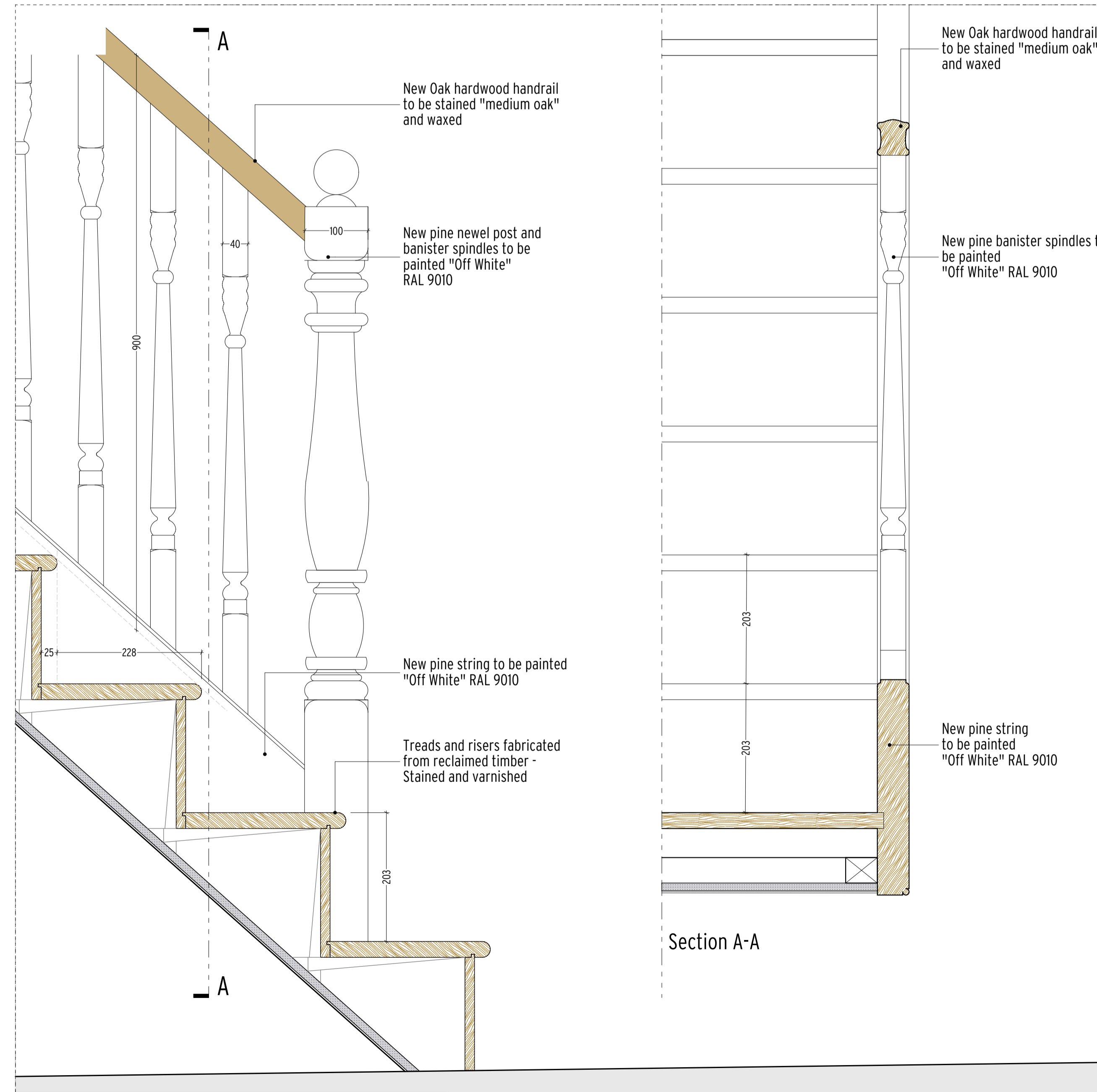
S5 & S6 Stair Typical Detail Scale 1:5 @ A1
