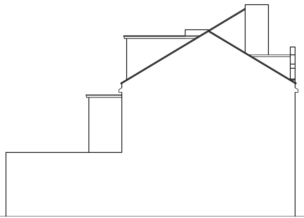
PRE-EXISTING SIDE ELEVATIONS
