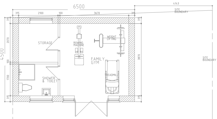
PROPOSED OUTBUILDING
