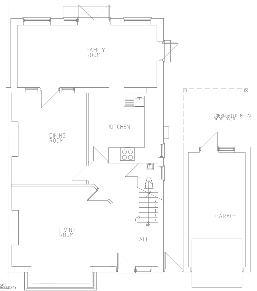
GROUND FLOOR PLAN (EXISTING)
