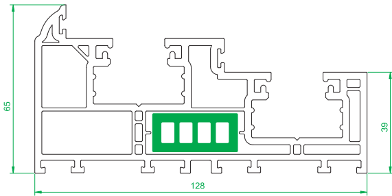
4001 Outer Frame
