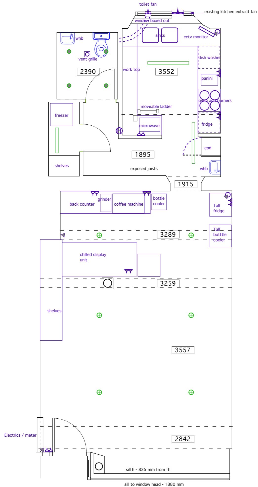
EXISTING PLAN- 1:50
