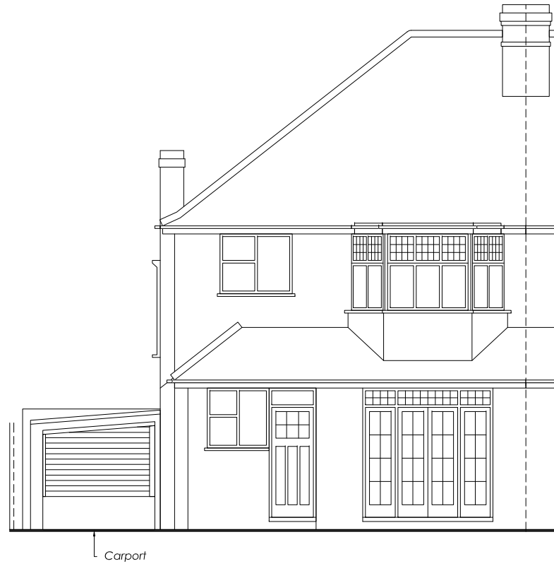
Rear Elevation
