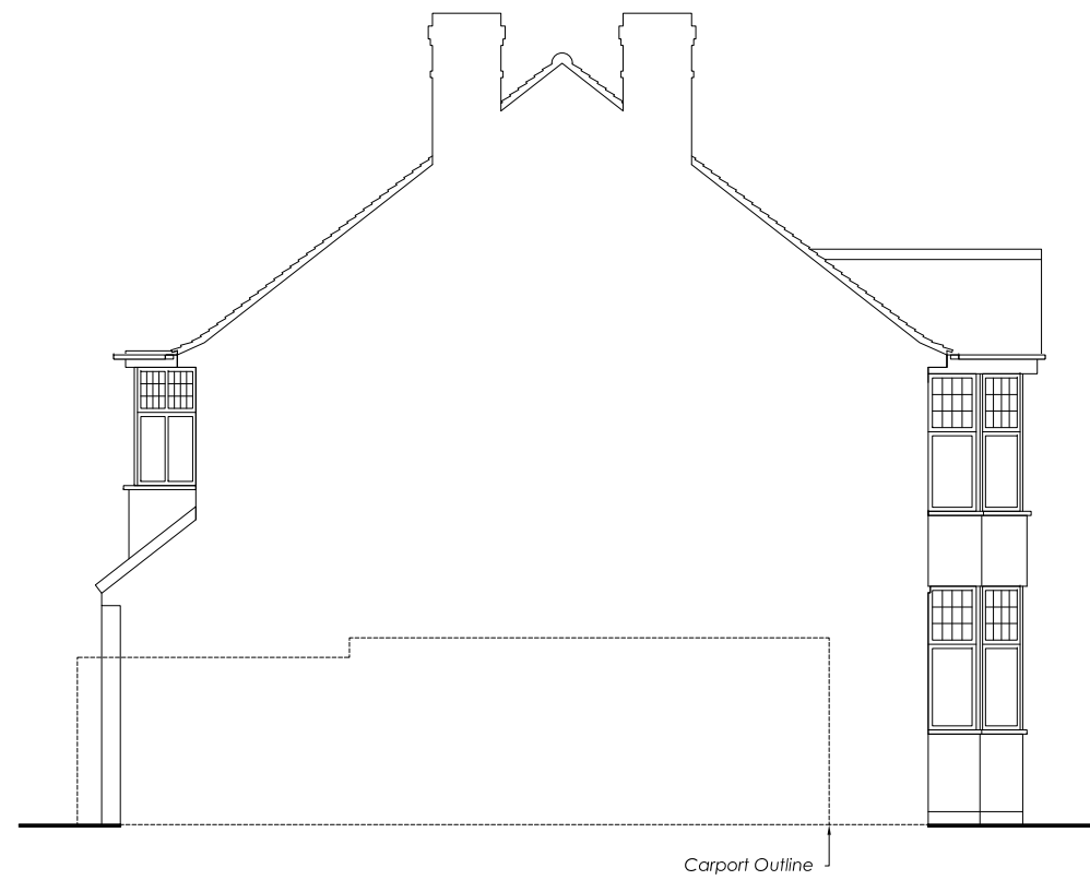
Side Elevation
