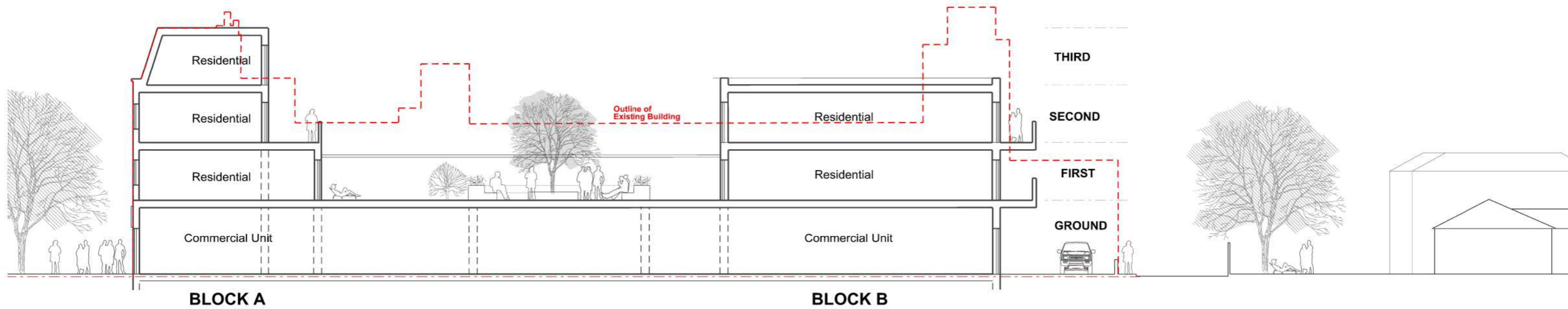
01. Proposed Section Scale 1:200
