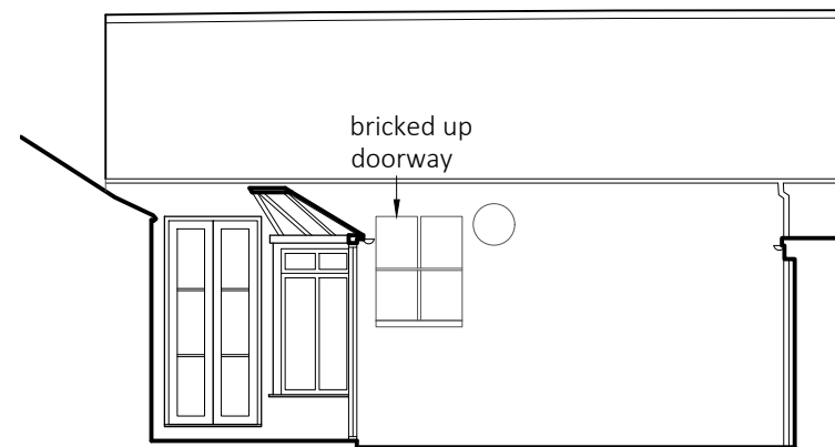
Courtyard Elevation (South)
