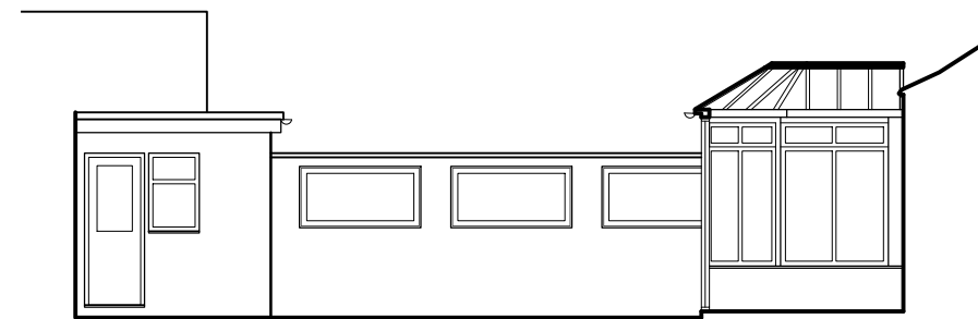
Courtyard Elevation (North)
