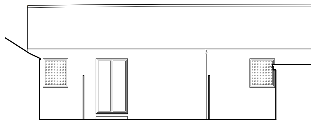
Courtyard Elevation (South)
