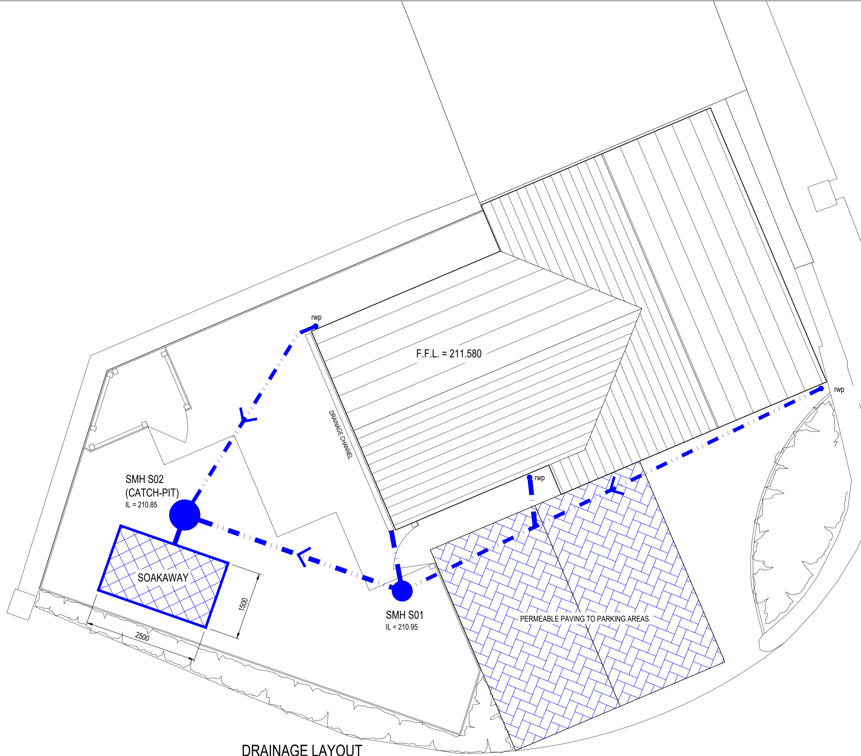
DRAINAGE LAYOUT SCALE 1:50
