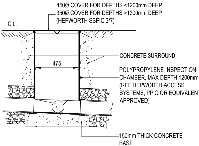
POLYPROPYLENE INSPECTION CHAMBER-PPIC
