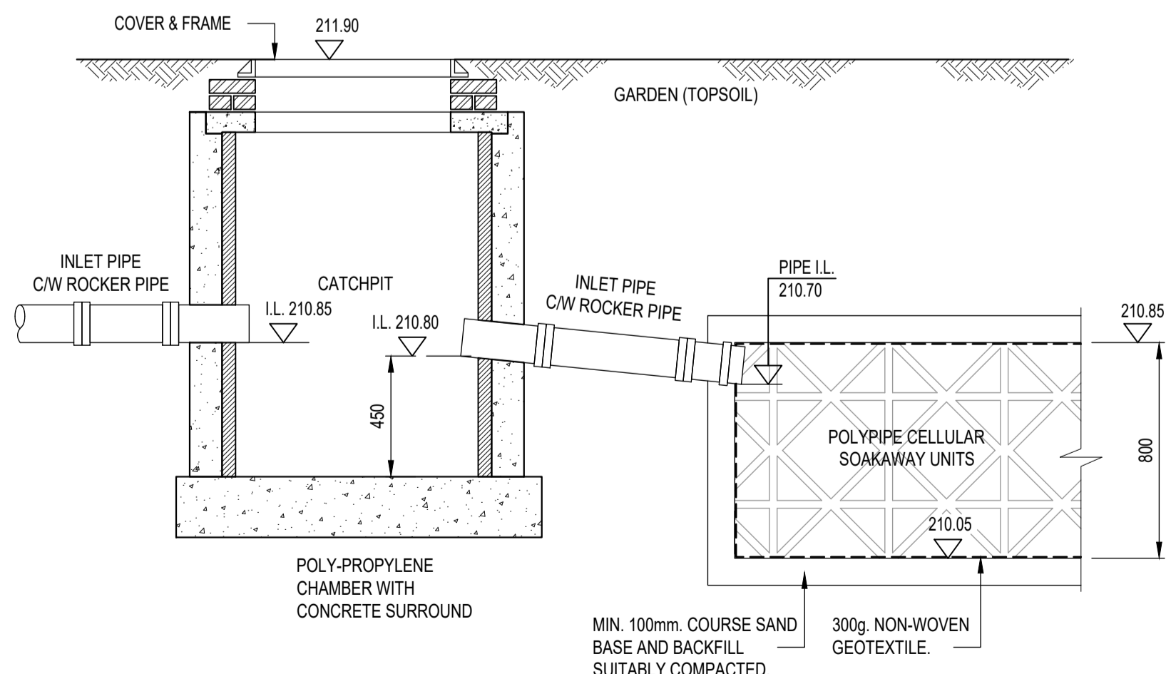
SECTION THRO' CATCH PIT & SOAKAWAY
