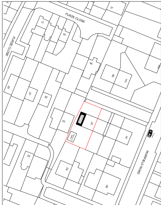
PROPOSED LOCATION PLAN 1:1250
