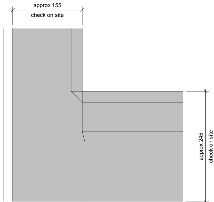
5 Architrave-Skirting Junction 1:5
