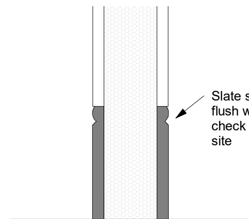
2 Skirting Type M 1:5
