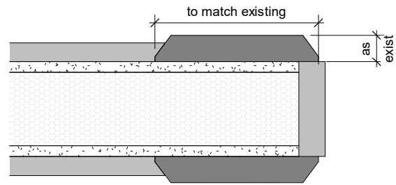
6 Architrave 1:5
