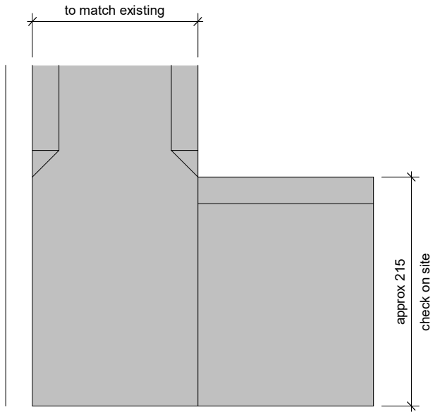
7 Architrave-Skirting Junction Copy 1 1:5
