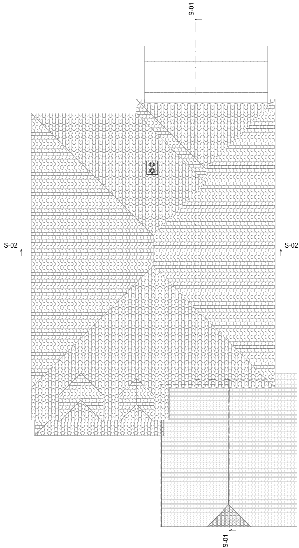
Roof Plan
