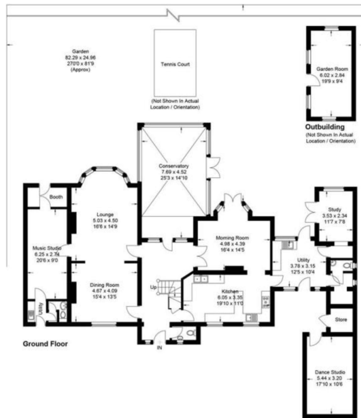
Ground Floor Plan as Existing
