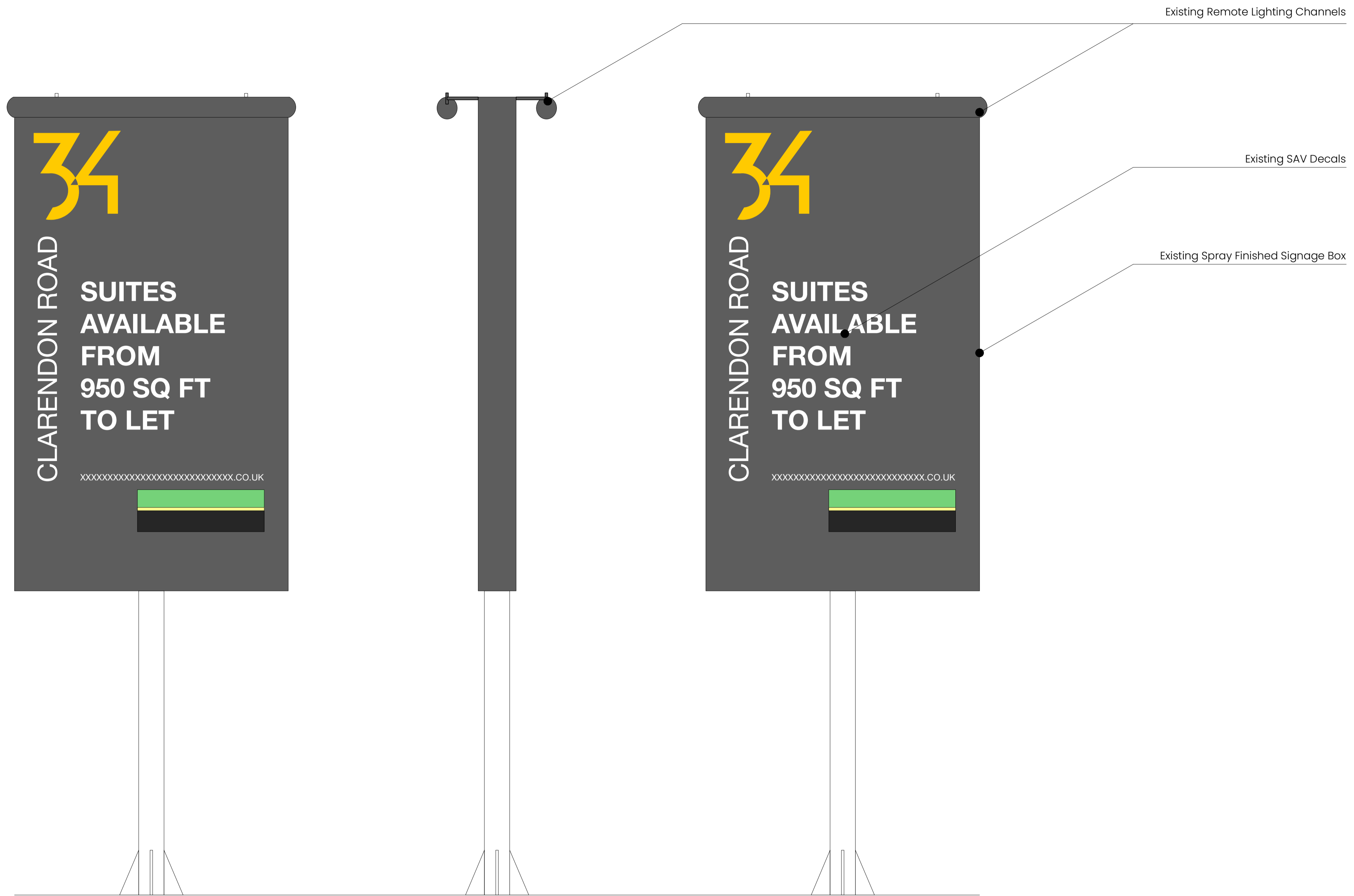
FRONT ELEVATION
