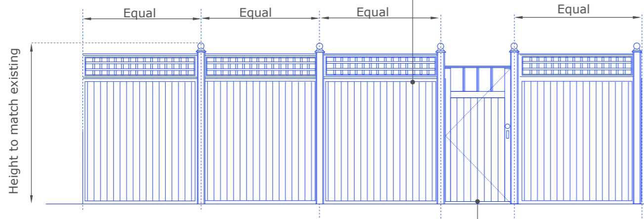
West Elevation - view from garden
