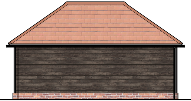
NORTH WEST ELEVATION - PLOT 5 NORTH EAST ELEVATION - PLOT 6
