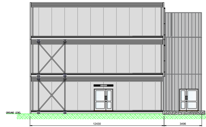
ELEVATION D
