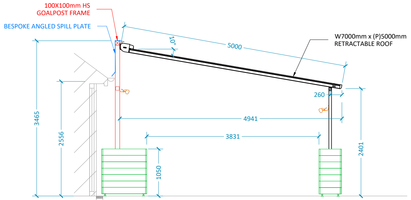
ELEVATION 1:100 B 161632-SQ39264-01
