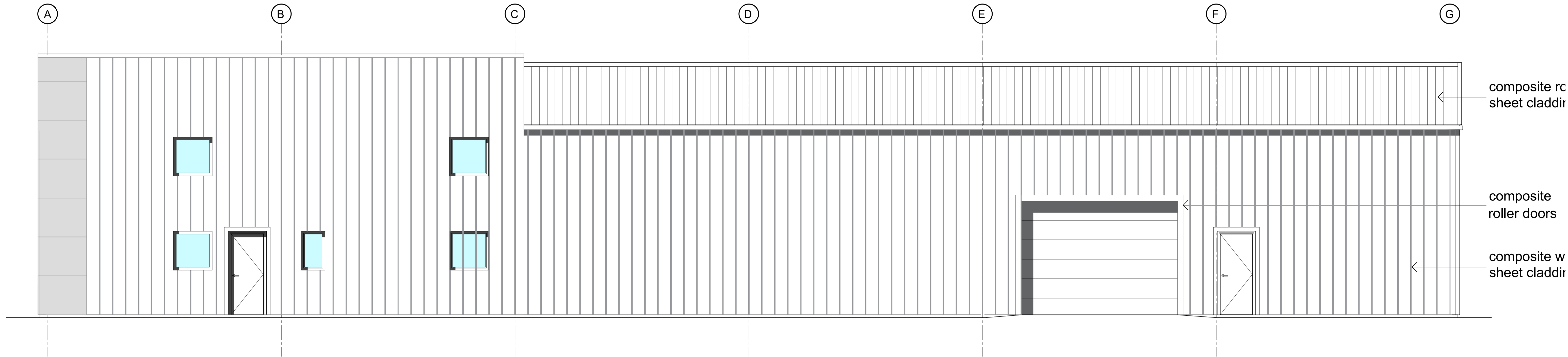
Proposed Side Elevation (North East)
