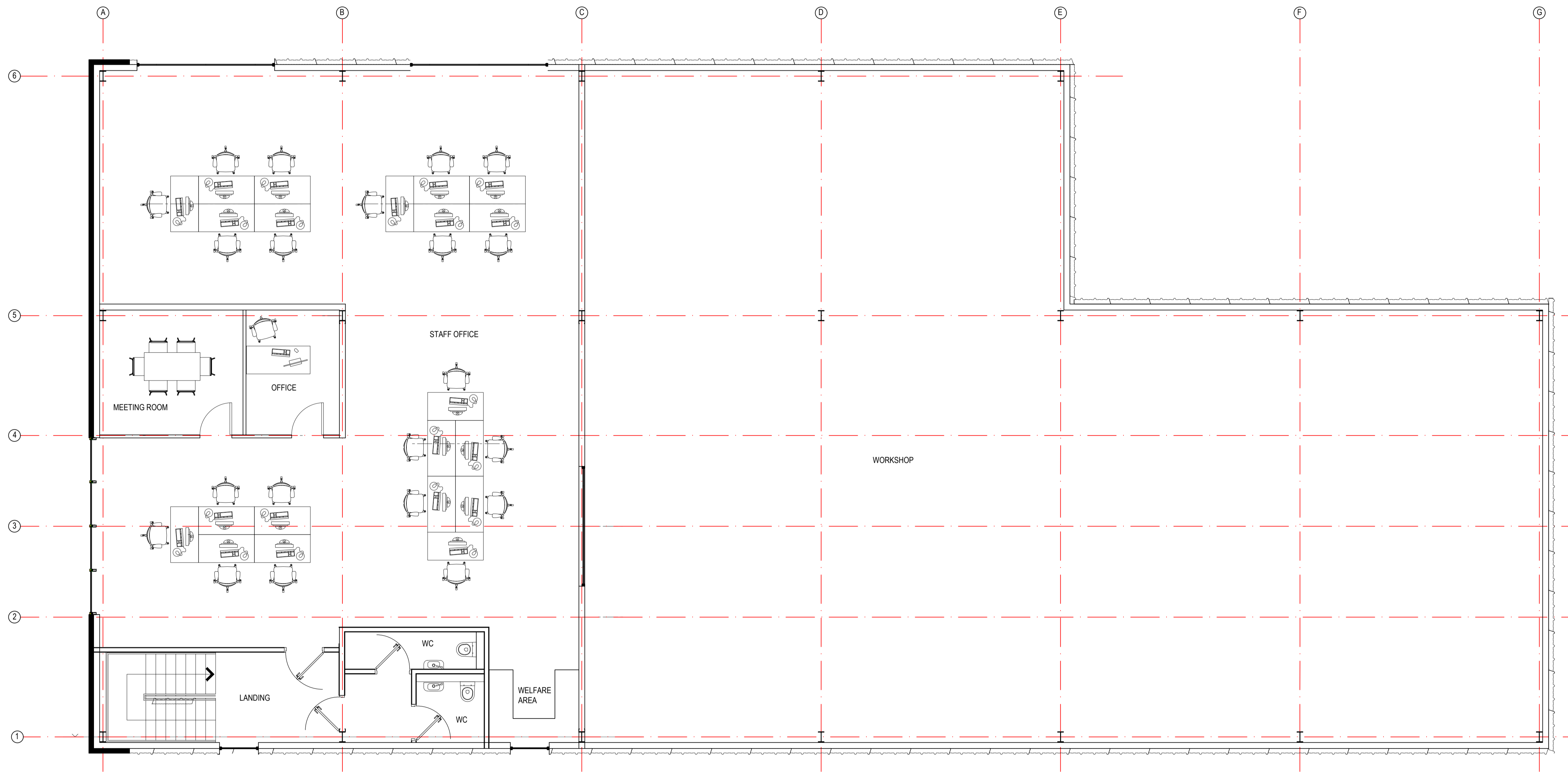
PROPOSED FIRST FLOOR PLAN
